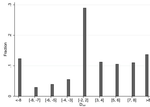
Figure 7: Distribution of \Delta_{s_r}
