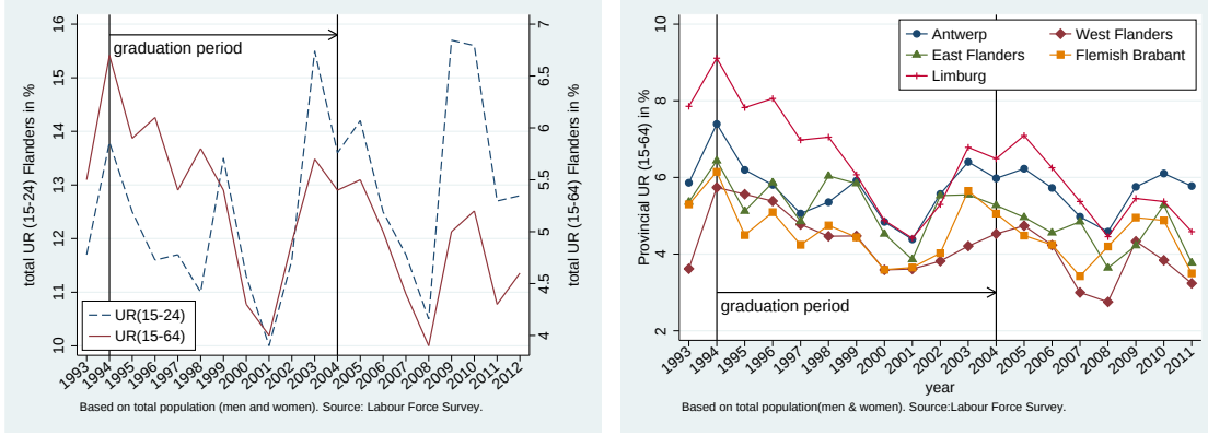
(a) National Unemployment Rates (UR): overall (age 15-64) and youth (age 15-24).
