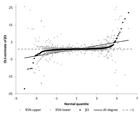
(f) \hat{\beta}_3 for (\alpha, \delta) = (-0.67, -0.25)
