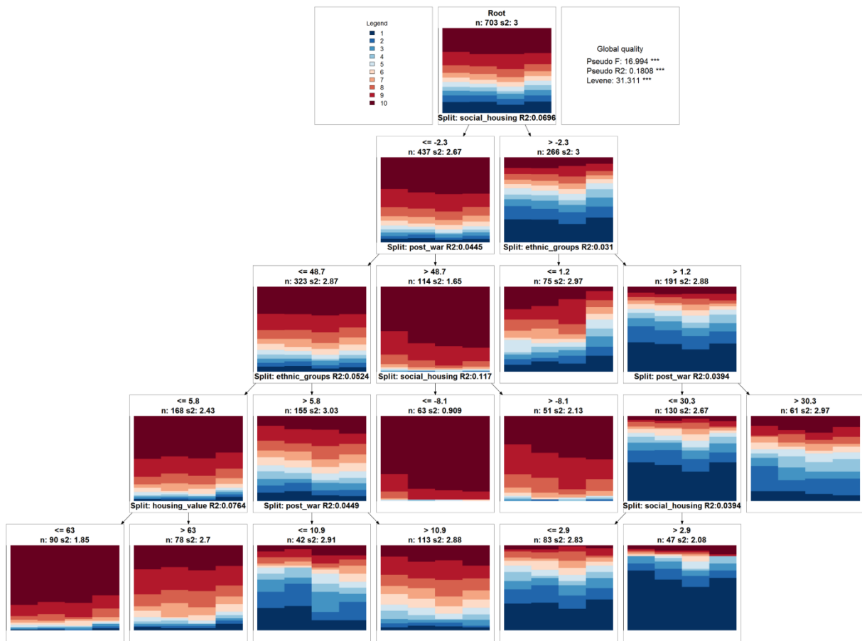
Figure 5 Tree-structured discrepancy analysis of neighbourhood trajectories
