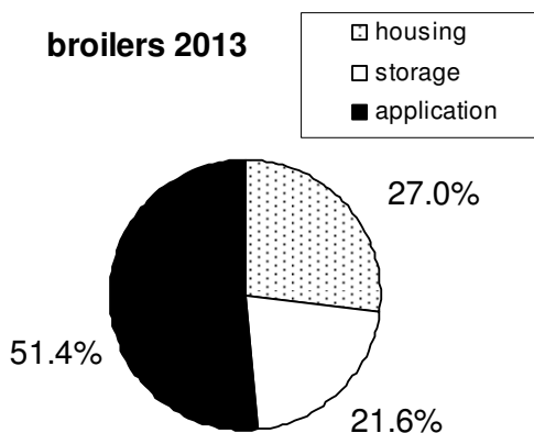
Figure 2.10: Broilers (Submission 2015): Percentages of \text{NH}_3 emissions originating from housing, storage, manure application and grazing in 2013
