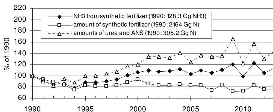
Figure 2.12: Application of mineral fertilizer N (amounts sold), amounts of N in urea and ANS applied, and the \text{NH}_3 emissions from the total application of mineral fertilizers (Submission 2015)
