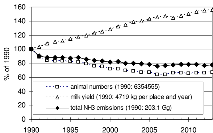
Figure 2.8: Development of dairy cattle numbers, milk yields and NH 3 from dairy cattle husbandry (including grazing), Submission 2015
