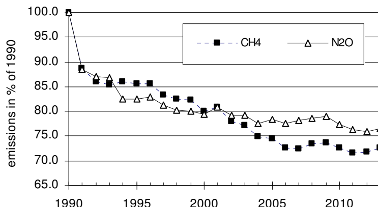
Figure 2.2: Development of CH 4 und N 2 O emissions from animal husbandry in % of 1990, Submission 2015 (enteric fermentation and manure management)
