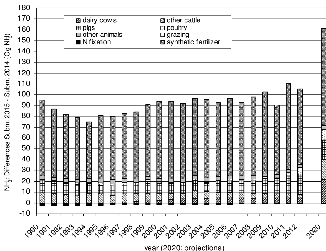
Figure 2.14: Differences of NH 3 emissions between Submission 2015 and Submission 2014
