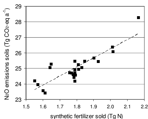
Figure 2.6: Total of annual N 2 O emissions (direct and indirect) from agricultural soils vs annual amounts of mineral fertilizer N for the years 1990 to 2013 (Submission 2015)
