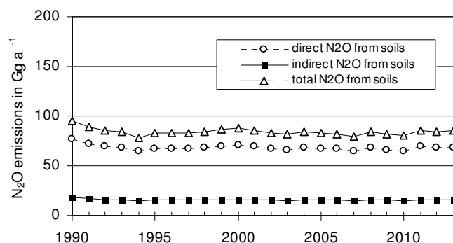
Figure 2.5: N 2 O emissions from agricultural soils (in Gg a -1 N 2 O), Submission 2015
