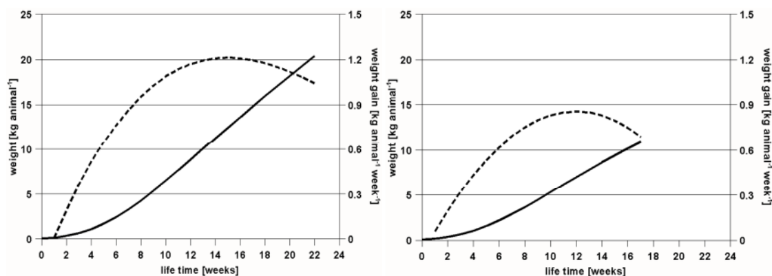
Figure 8.3: Turkeys, typical animal weight and weight gain developments
