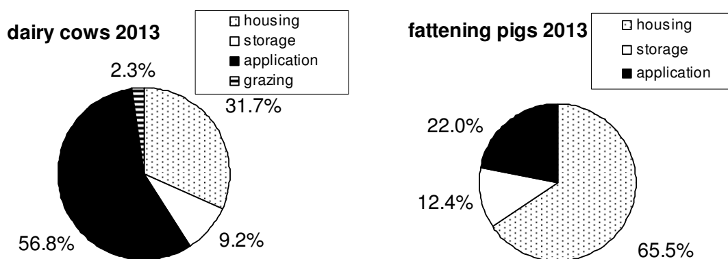
Figure 2.9: Dairy cows and fattening pigs (Submission 2015): Percentages of \text{NH}_3 emissions originating from housing, storage, manure application and grazing in 2013 (no free range husbandry for pigs)
