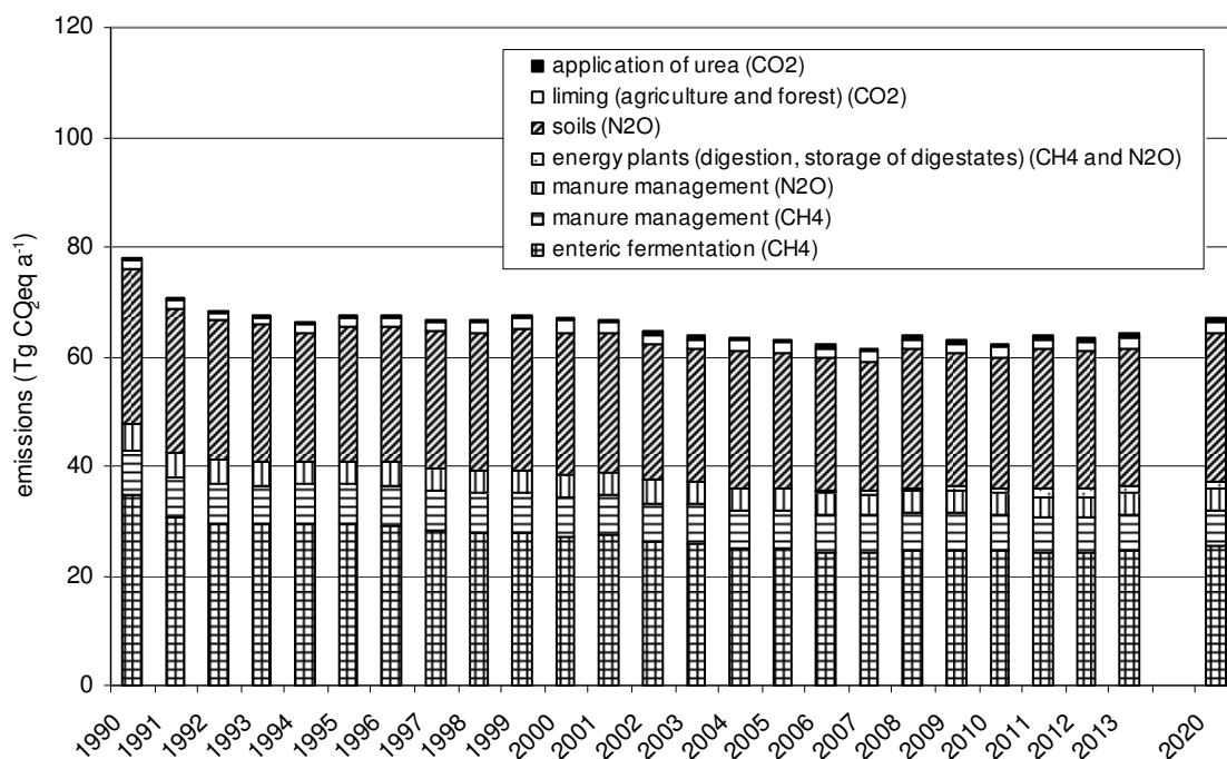
Figure 2.1: Annual THG emissions from German agriculture and projections for 2020 (Submission 2015) (GWP: CH 4 25, N 2 O 298)
