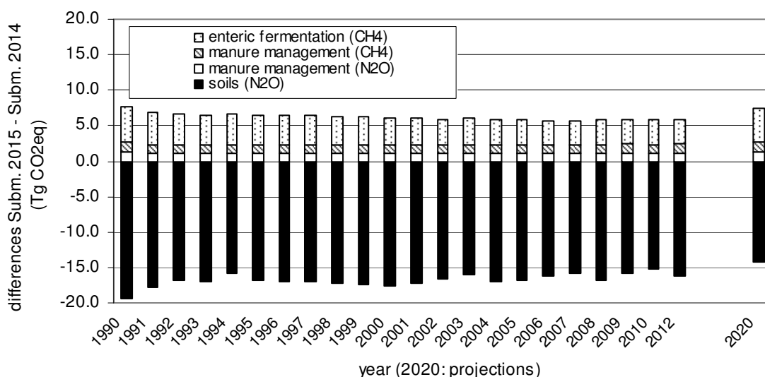
Figure 2.13: Differences of THG emissions between Submission 2015 and Submission 2014
