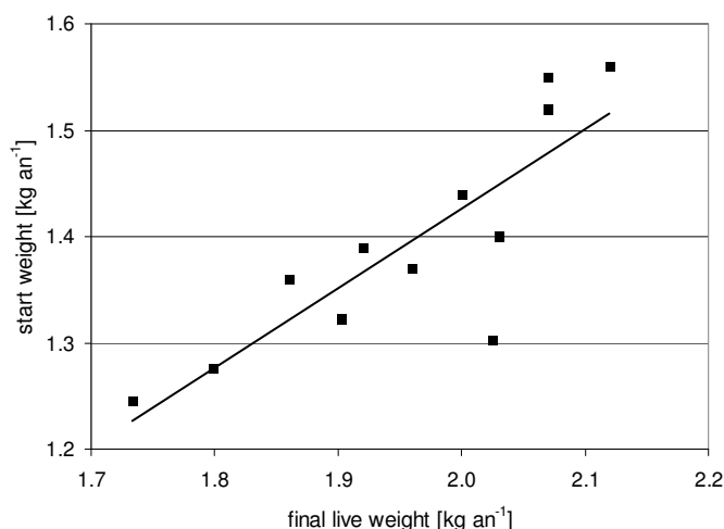
Figure 8.1: Laying hens, relation between weight at the beginning of egg production period and final live weight
