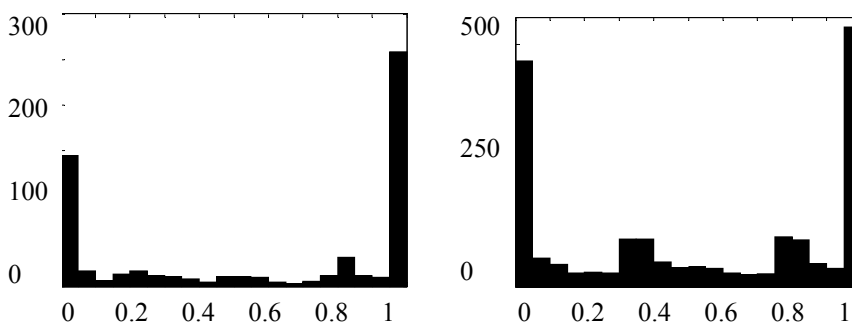
Fig. 3: Histograms of ultimate recovery rates on the data sets D1 (left) and on D3 (right)
