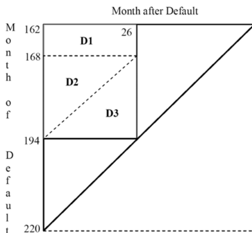
Fig. 2: The original and modified data sets
