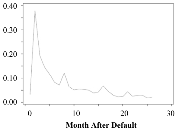
Fig. 4: The baseline hazard function given by the Cox regression
