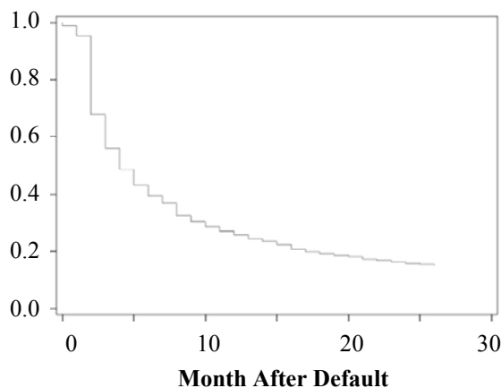
Fig. 5: The survival function for the first account given by the Cox regression
