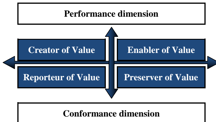
Fig. 3: Controllers' Roles
