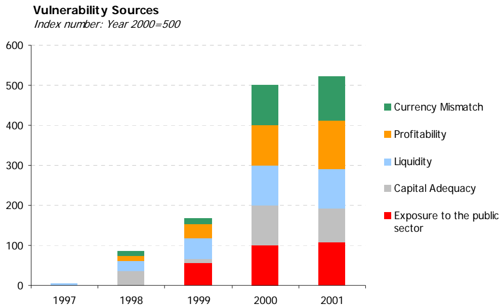
Figure 4: Vulnerability Sources
