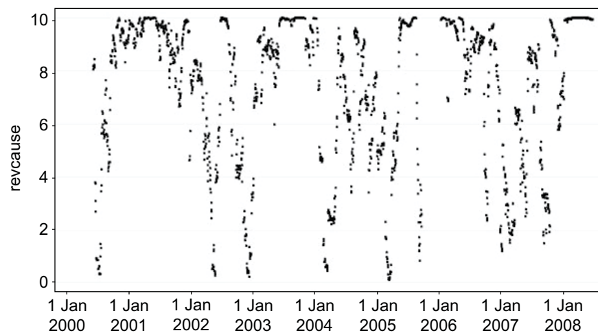
Appendix Figure 3.10: Hard Wheat \Leftarrow Rice
