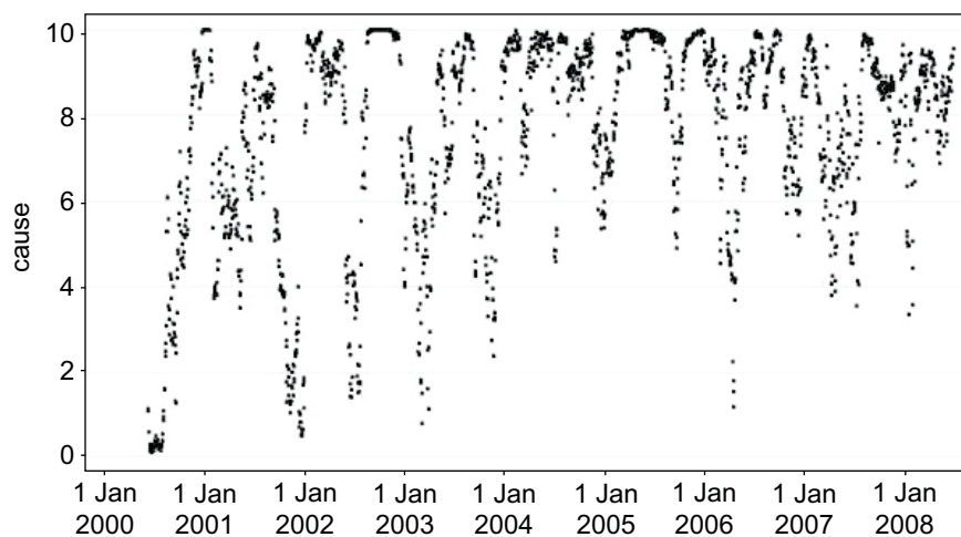
Appendix Figure 3.5: Oil (Brent)⇒Corn (Maize)
