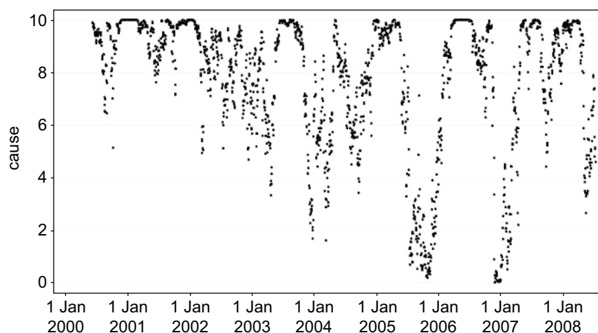
Appendix Figure 3.1: Euro/US$⇒Brent Crude
