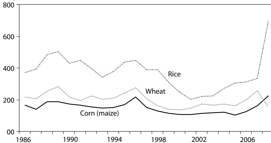
Figure 1: Short-Run Movements in Real Prices of World Grains ($ per metric ton)
