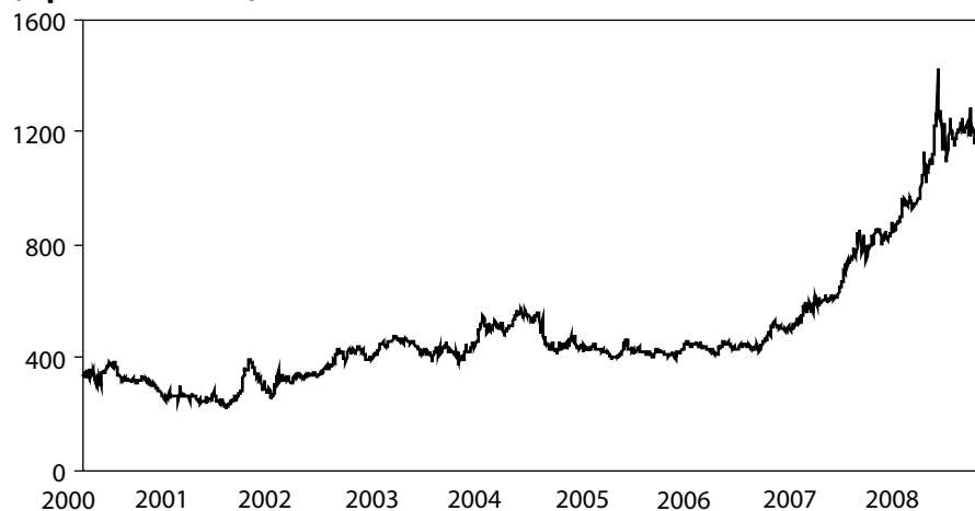
Figure 8: Palm Oil Price Movements
