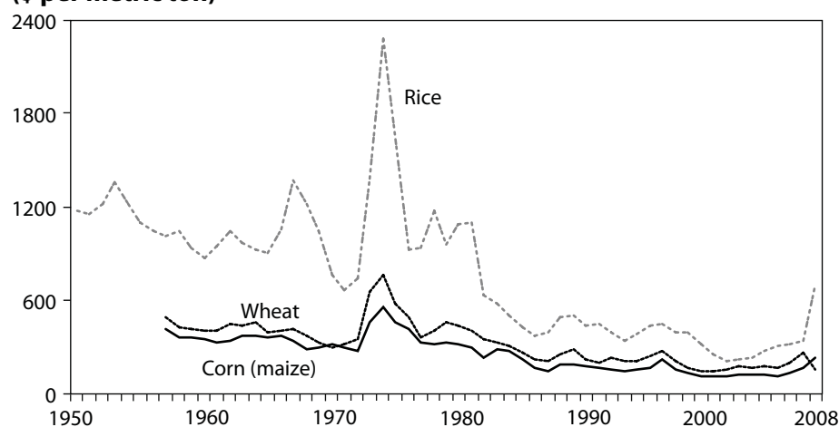
Figure 2: Long-Run Movements in Real Prices of World Grains
