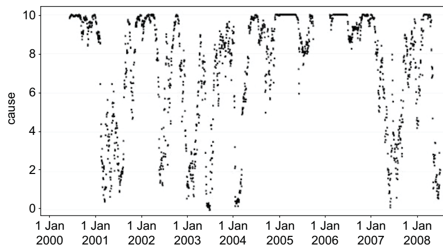
Appendix Figure 3.9: Hard Wheat \Rightarrow Rice
