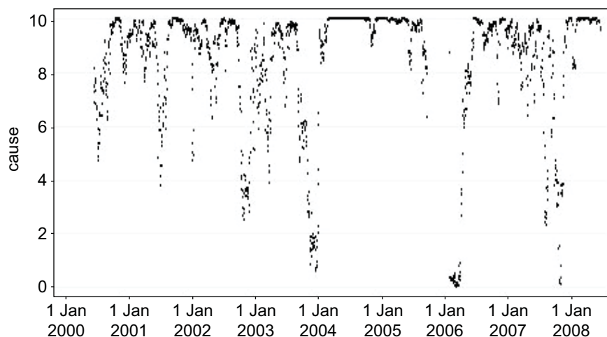
Appendix Figure 3.4: Euro/US$⇒Rice
