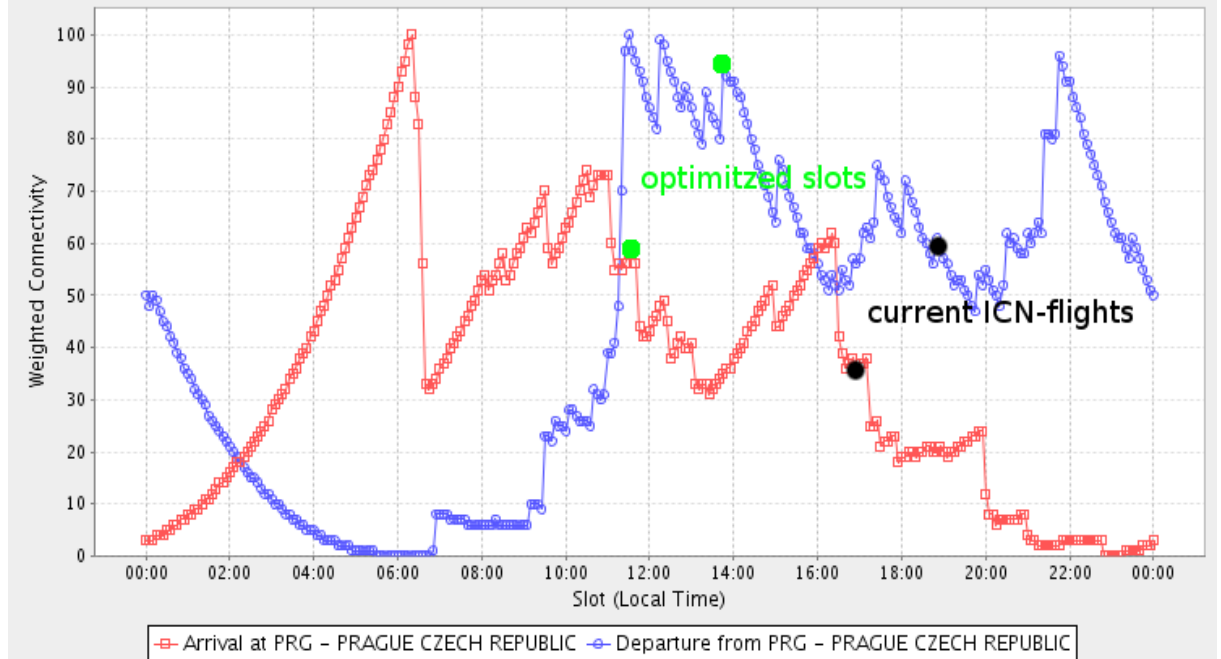
Arrival/departure from ICN at PRG versus demand
