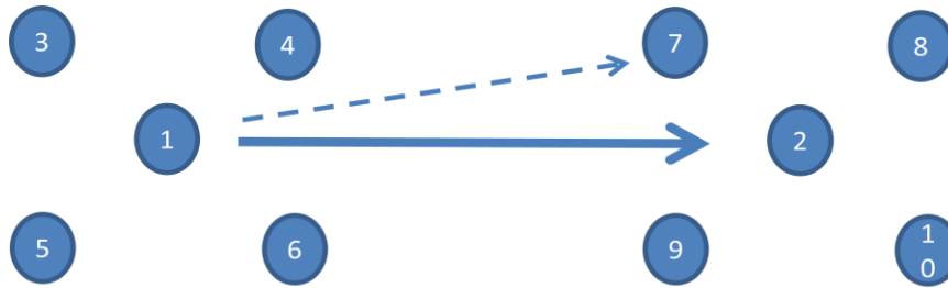
Figure 3. Spatial competition
