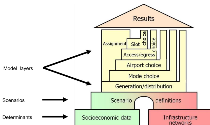
Figure 2. Sequence of models for air transport forecasting
