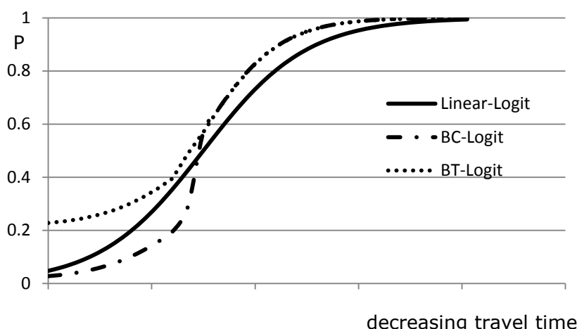
Figure 4. Functional forms
