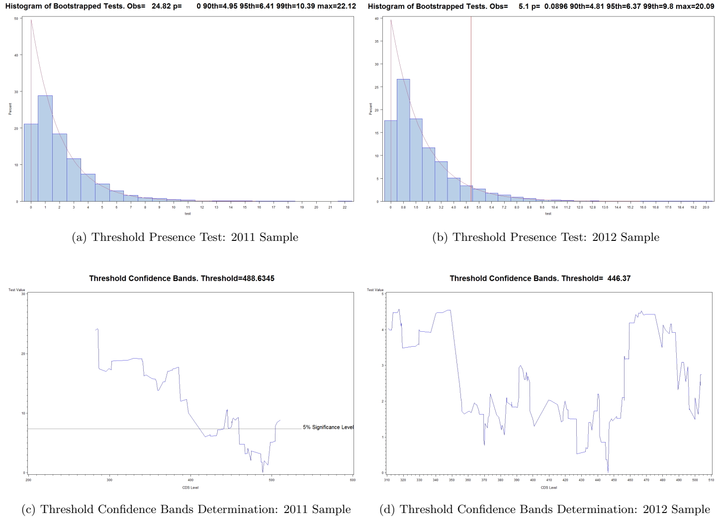
Figure 11: Bootstrapped Threshold Significance Test Distribution and Confidence Bands Determination for Two Subsamples. We bootstrapped the distribution of the test for the presence of a threshold and plot the distribution in Panels (a) and (b) for the sub-samples before and after the structural break, respectively. The vertical red lines mark the observed test values, while the curve superimposed on the empirical distribution is a chi-square distribution with as many degrees of freedom as parameters that are allowed to change in the specification, for reference. The test statistic described in Appendix C is plotted here for Equation 4 in Panels (c) and (d) for the sub-samples before and after the structural break, respectively. The test statistic is normalized at 0 at the threshold that minimizes the sum of squared residuals. The horizontal line at 7.35 marks the 5% confidence values for the threshold.
