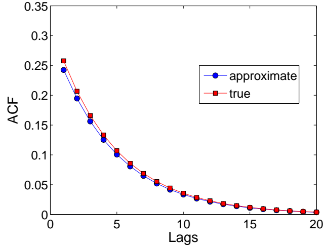
Figure 5: ‘True’ and approximate autocorrelation functions of the z_t^2 -process.
