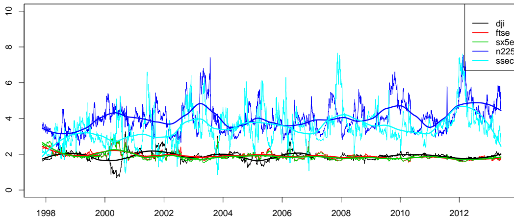
Figure 8: Relative entropy, different shock origins
