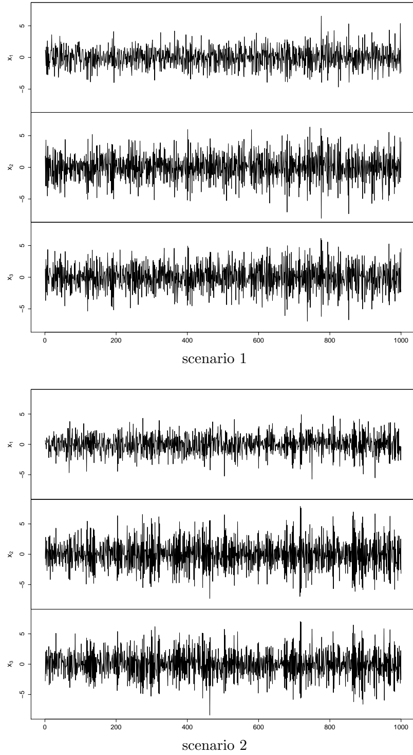
Figure 6: Time-varying spillover patterns: simulation results
