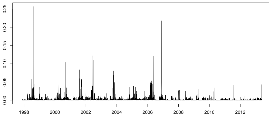
Figure 9: Relative entropy, day by day, stationary case
