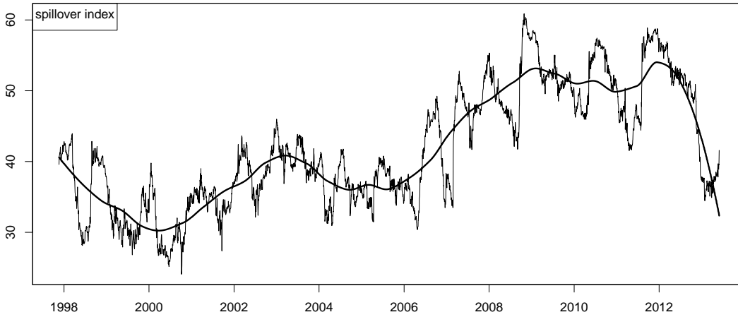
Figure 3: The spillover index series, the case dji/ftse/sx5e/n225/ssec
