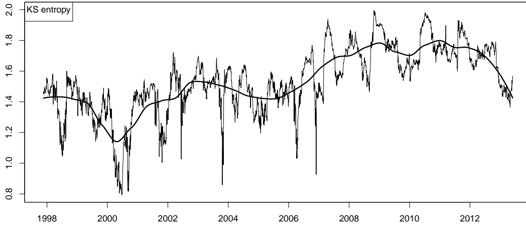
Figure 10: Relative entropy, day by day, non-stationary case
