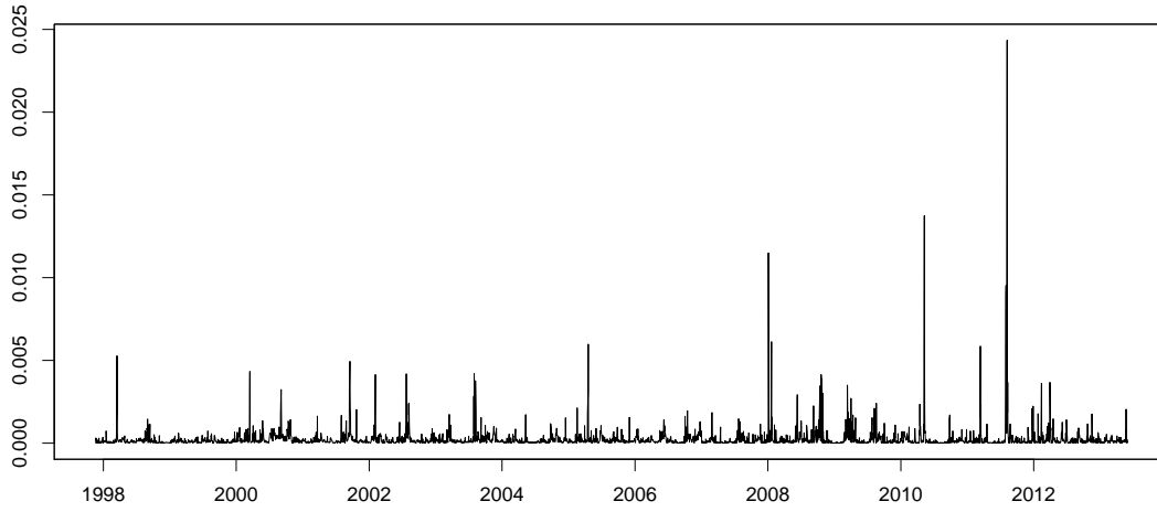
Figure 10: Relative entropy, day by day, non-stationary case
