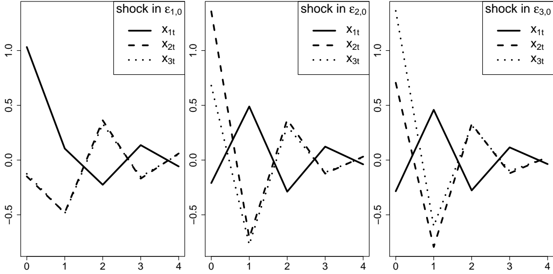
Figure 4: An impulse response function reproducing the spillover table in example (b)
