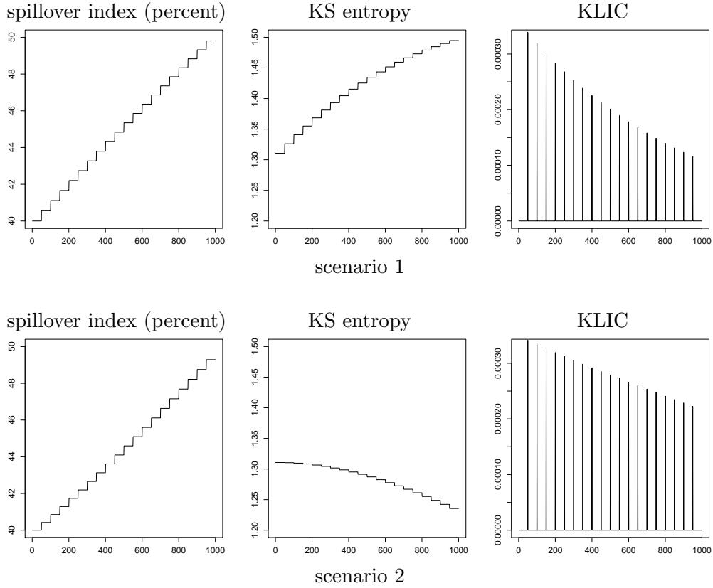
Figure 5: Time-varying spillover patterns: two scenarios
