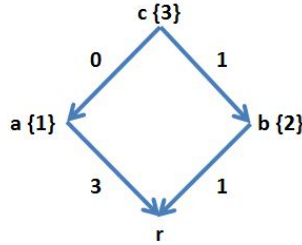
Figure 3: The supermodularity of the characteristic function
