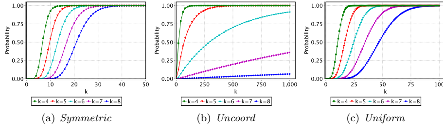
Figure 1: Probability of reaching a stable matching within R rounds.
