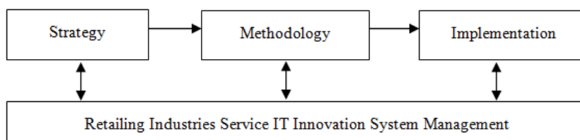
Figure 3: Implementation Model
