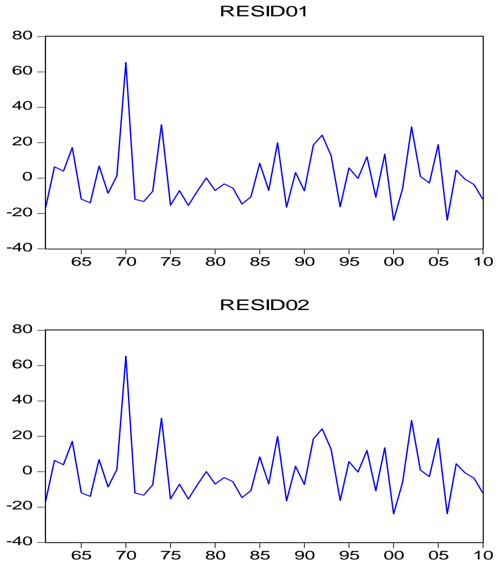
Figure 1 Graphs of the Residuals showing the stationarity properties
