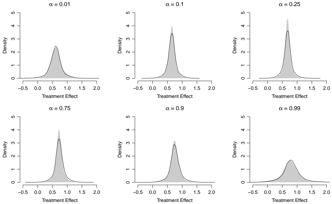
Figure 1: Distribution of the cETE (grey area) and cQTE (solid black line) of a simulated treatment effect \mu_{Z,1} = 0.7 at various locations \alpha .
