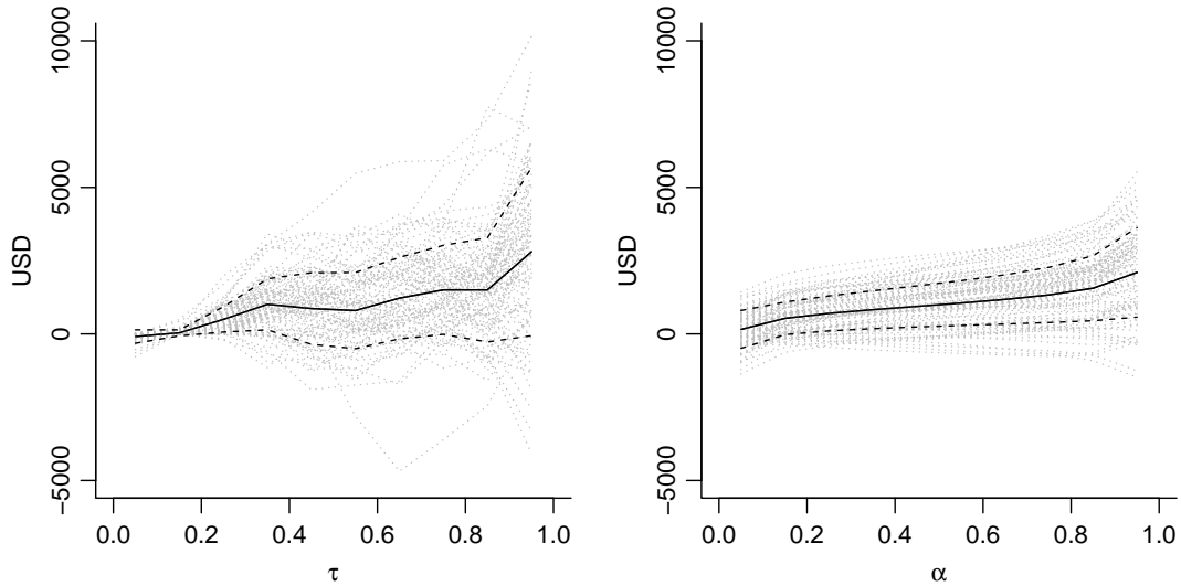
Figure 2: Mean (black solid line) and standard deviation (black dashed line) from the distribution of the treatment effect from QTE (left) and ETE (right) accompanied by 100 random draws (grey dotted lines) from the 1000 bootstrap runs.
