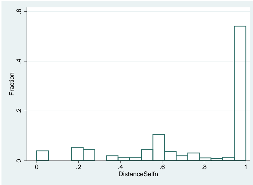
Figure 7: Selfn Distribution
