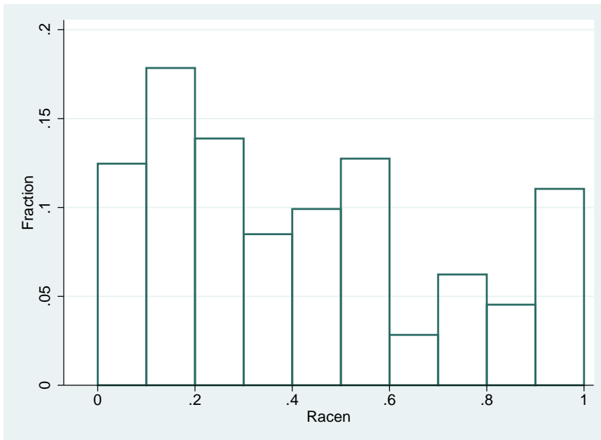
Figure 8: Racen Distribution
