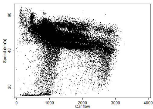
Figure A4 – Speed-flow relationship inner city roads
