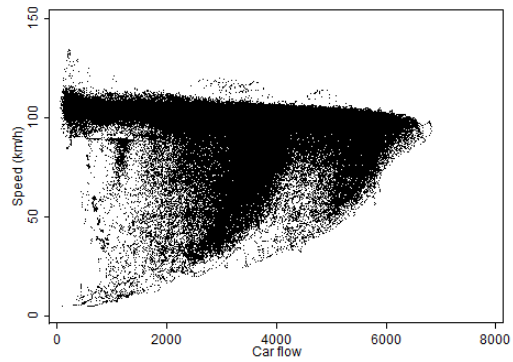
Figure A5 – Speed-flow relationship highway
