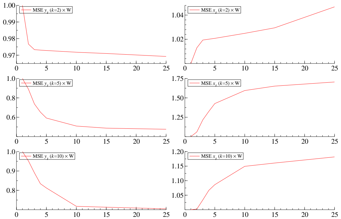
Figure 4: Scenario 2: Misspecification
