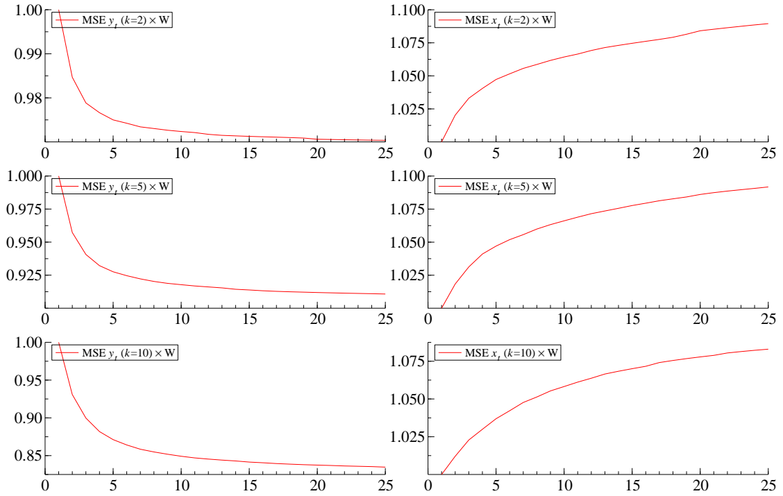
Figure 3: Scenario 1: Underspecification
