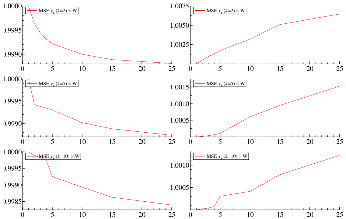
Figure 5: Scenario 3: Correct specification
