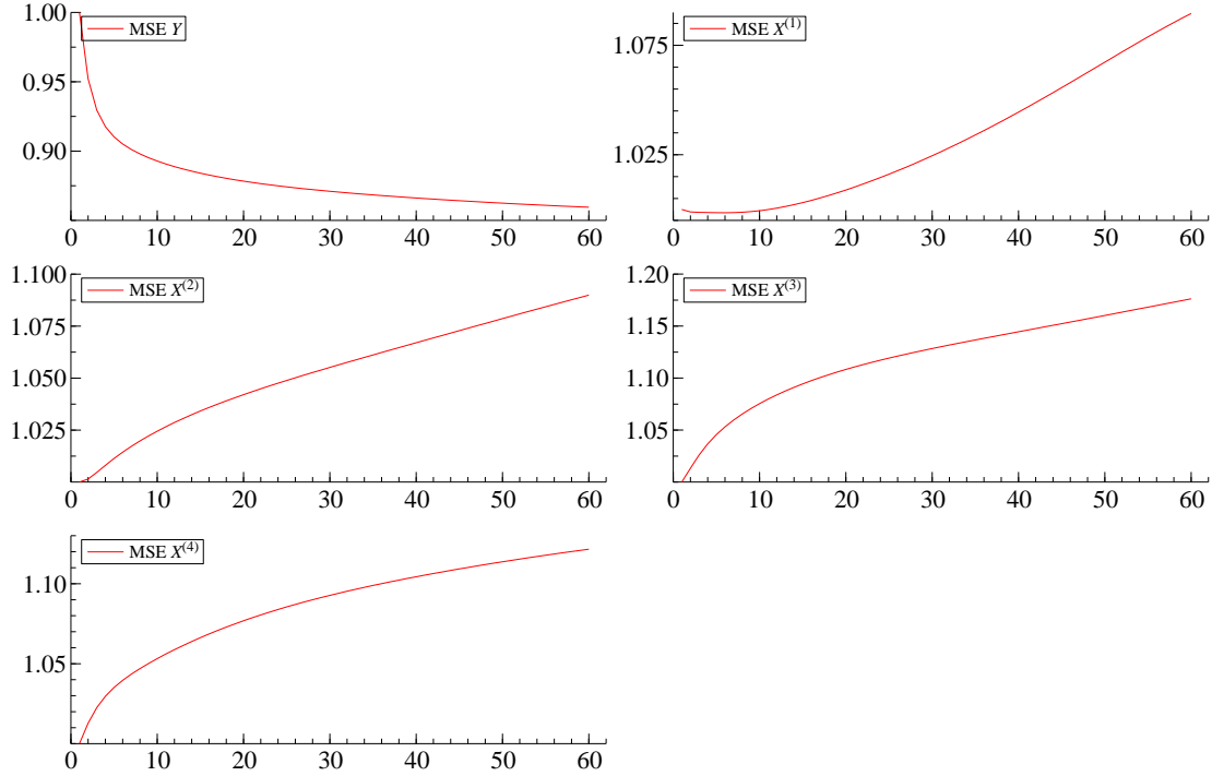
Figure 2: In-sample accuracy using WML
