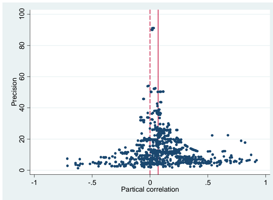
Figure 1: Funnel plot of growth-FDI partial correlations, all data (n = 946)
