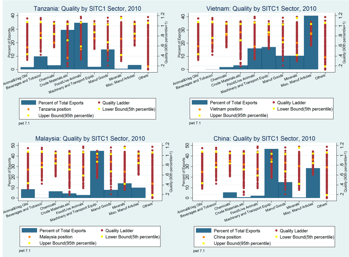
Figure 5. Quality ladders
