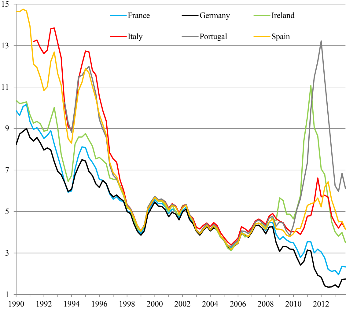
Figure 1: Long-term yields in percent of selected countries from 1990 to 2013.
