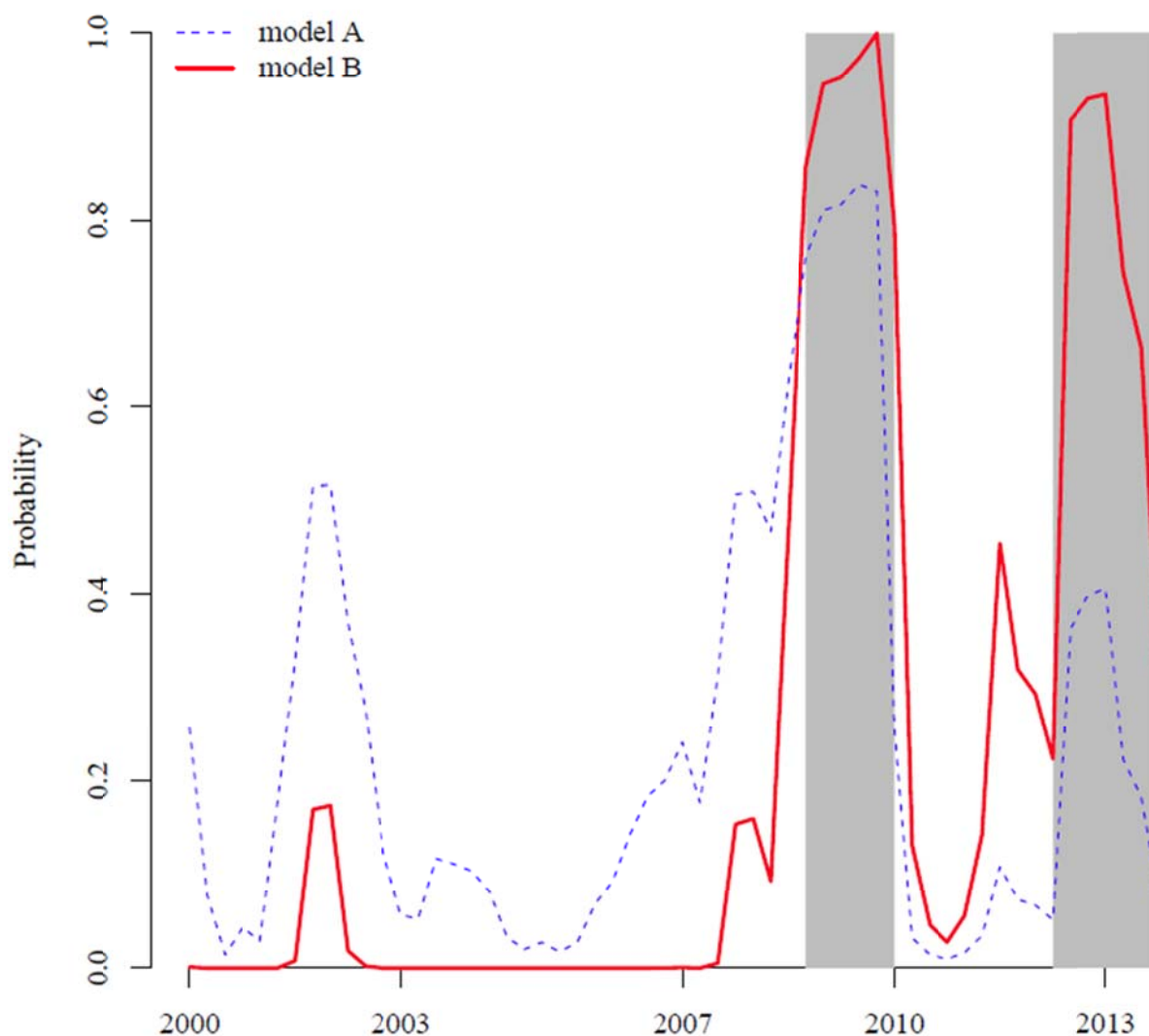
Figure 3: Predicted probabilities of recession and actual recessions in the Eurozone.
