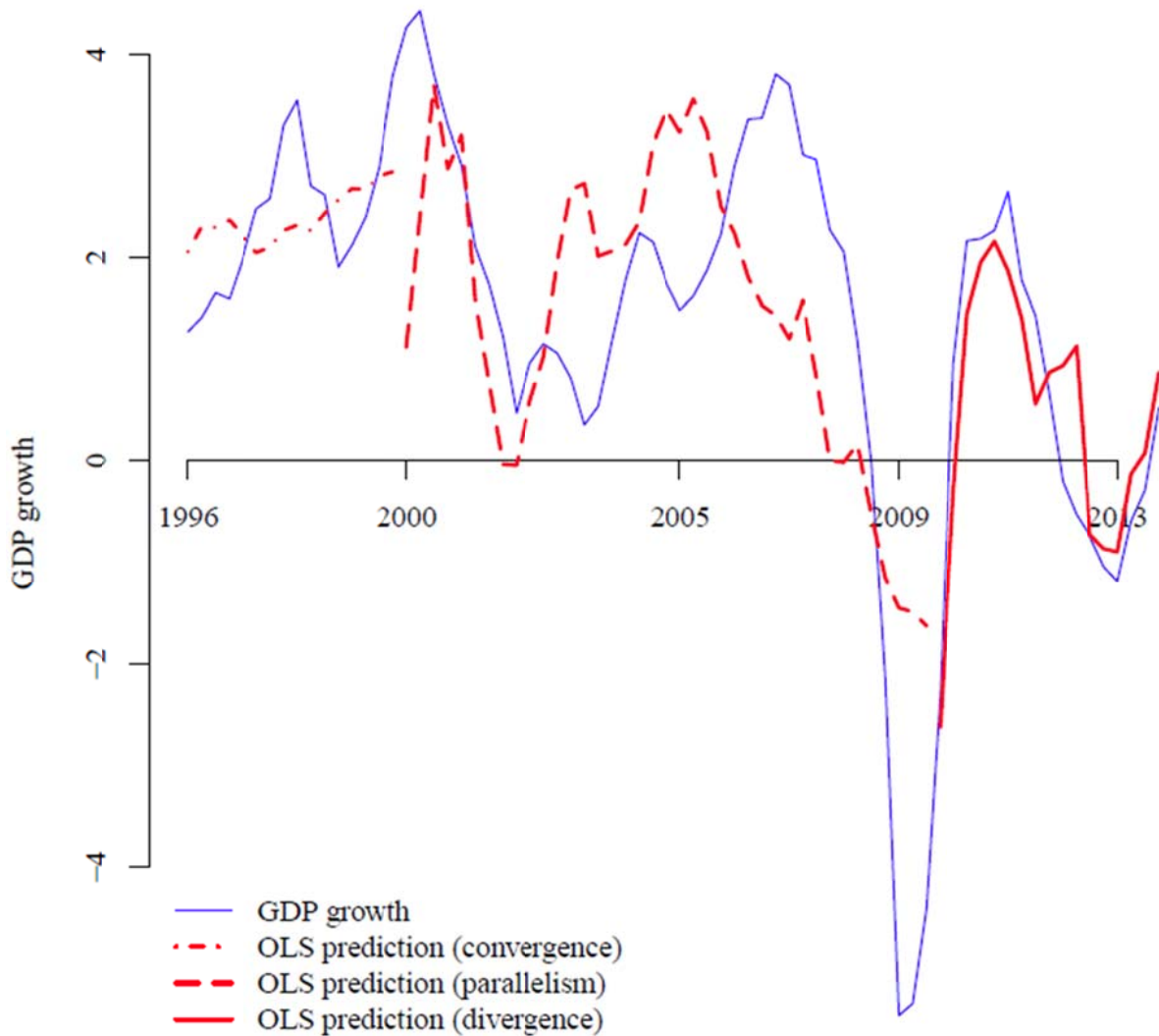
Figure 2: Estimated and real values of real GDP growth in percent in the Eurozone.
