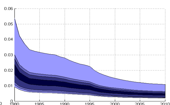
(f) Precision of beliefs (expectations)
