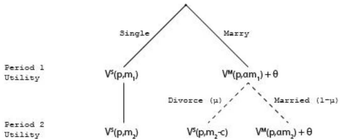
Figure 1: Decision Tree
