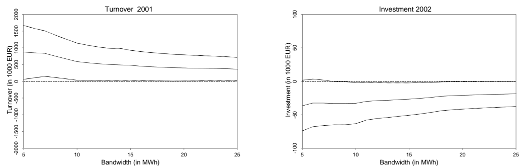
Figure 11: The effect of bandwidth choice on point estimates and confidence intervals.
