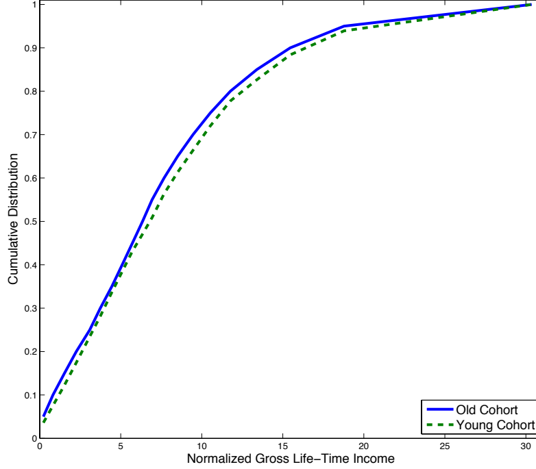
Figure 6: The estimated cumulative distribution of gross life-time income for the two cohorts. Note: Normalized income is defined as the annuatized (one period is five years) value of life time income in 10,000$ of 1980.
