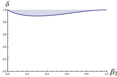
Figure 5: Region where e_2^T = \frac{V}{c} can be Attained
