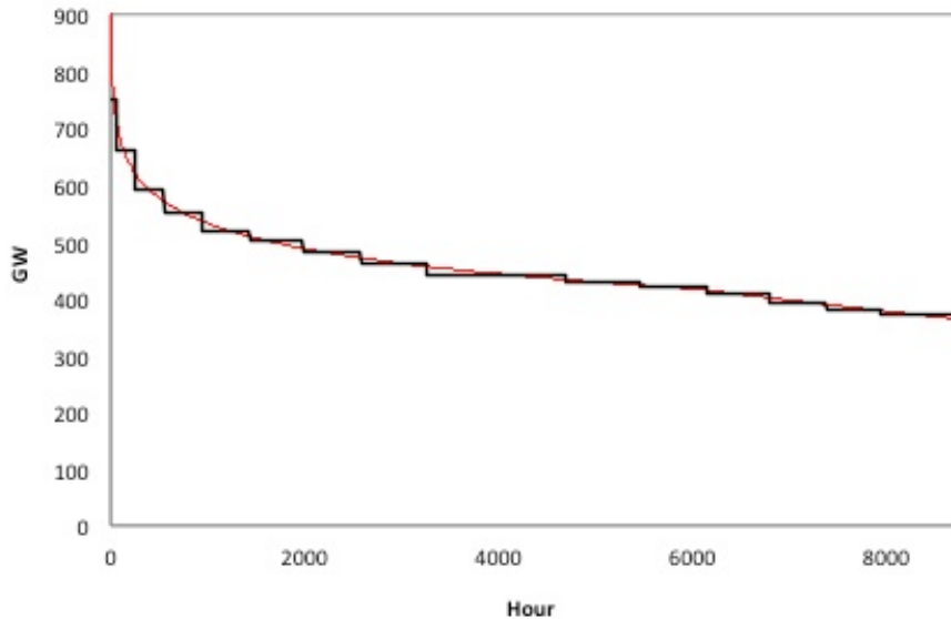
Figure 1. Load Duration Curve Used (Original Source: Short et al. 2009)
