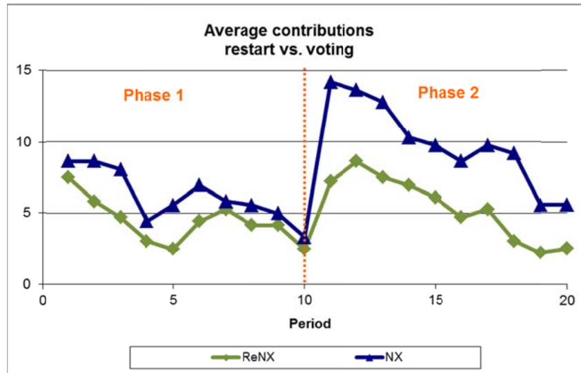
Figure 5 Robustness Check
