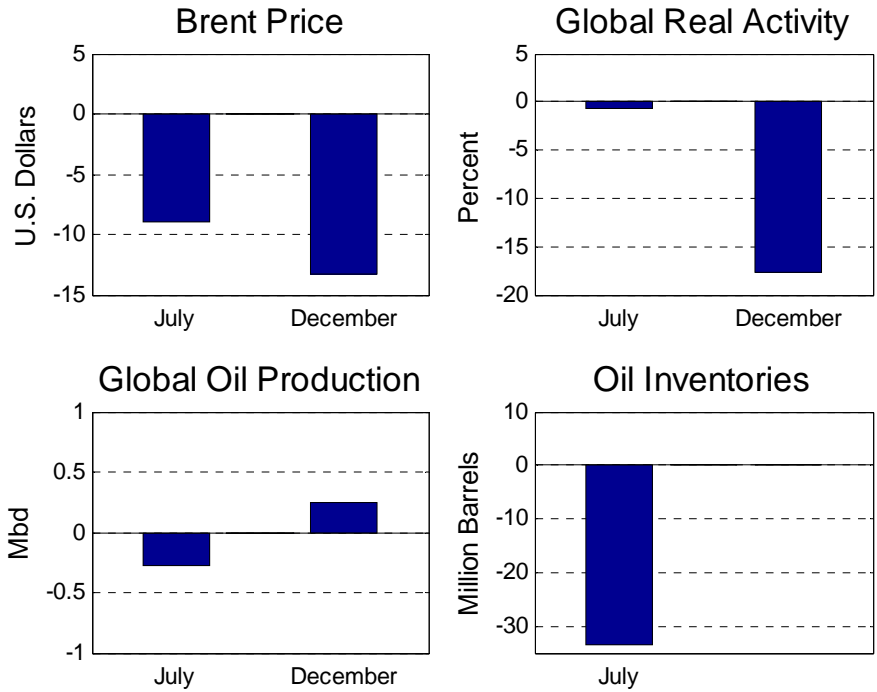
Figure 3: 1-Step-Ahead Forecast Errors for July 2014 and December 2014
