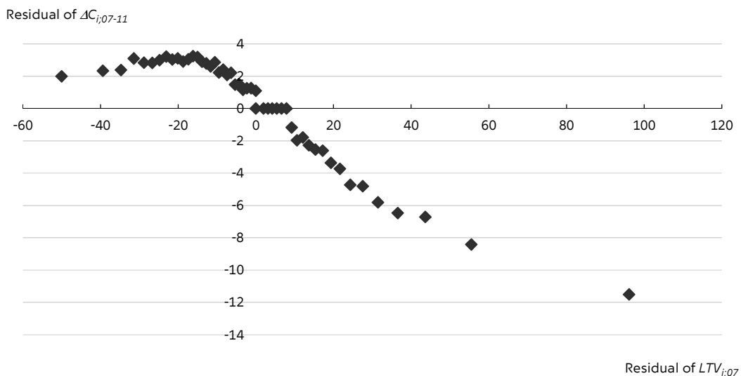
Chart 3: Binned residual plot. LTV ratio in 2007 and change in consumption from 2007 to 2011
