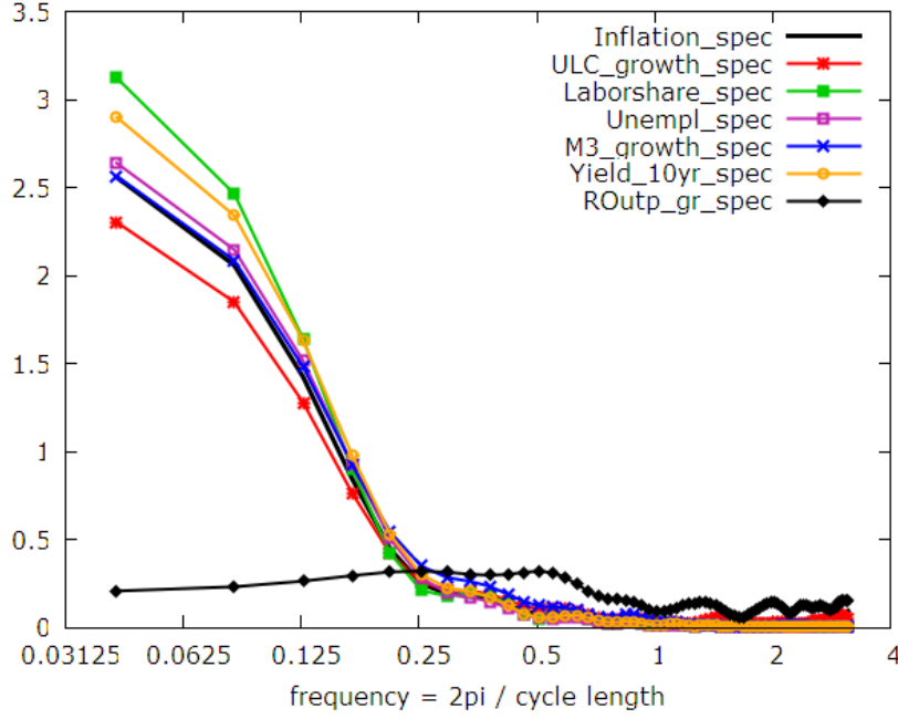
Figure 5: Spectra of the variables. The frequency axis is given in logarithmic scale to emphasize the low-frequency portion. Variables were normalized to have unit variance.
