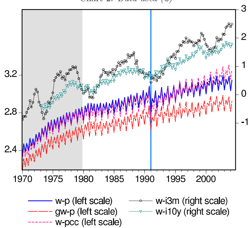
Chart 2: Data used (2)
