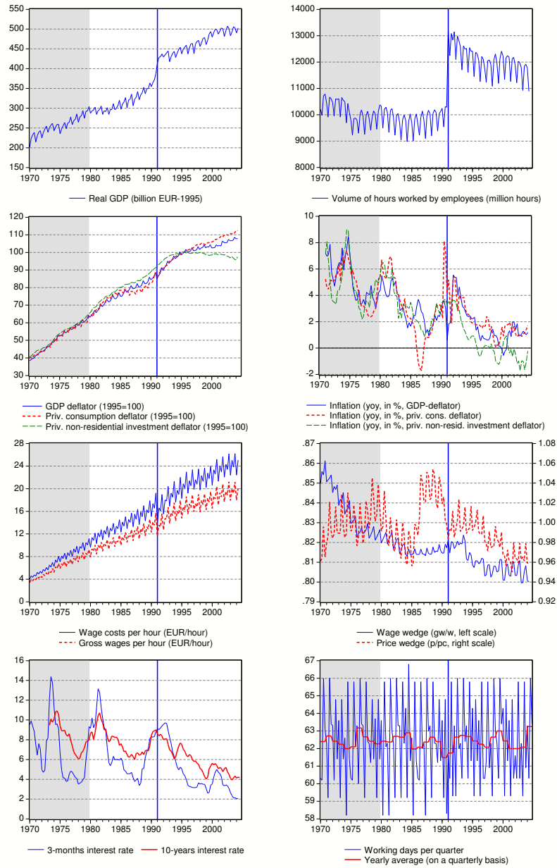
Chart 1: Data used (1)
