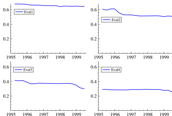
Figure 3: Recursive eigenvalues
