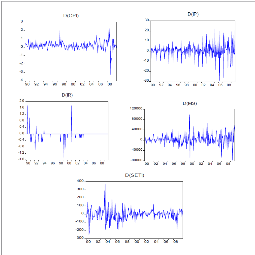
Figure 3. Graphical illustrations of the variables (at first difference)
