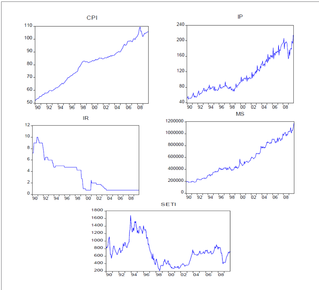
Figure 2. Graphical illustration of the variables (at level)
