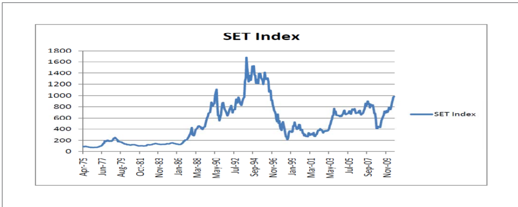
Figure 1. Thailand SET Index Monthly Movement, 1975-2010
