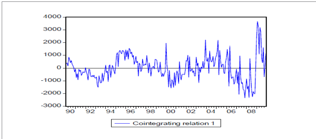
Figure 4. The Long-term movements between the Thai Stock Index (SETI) and the Selected Macroeconomic Variables
