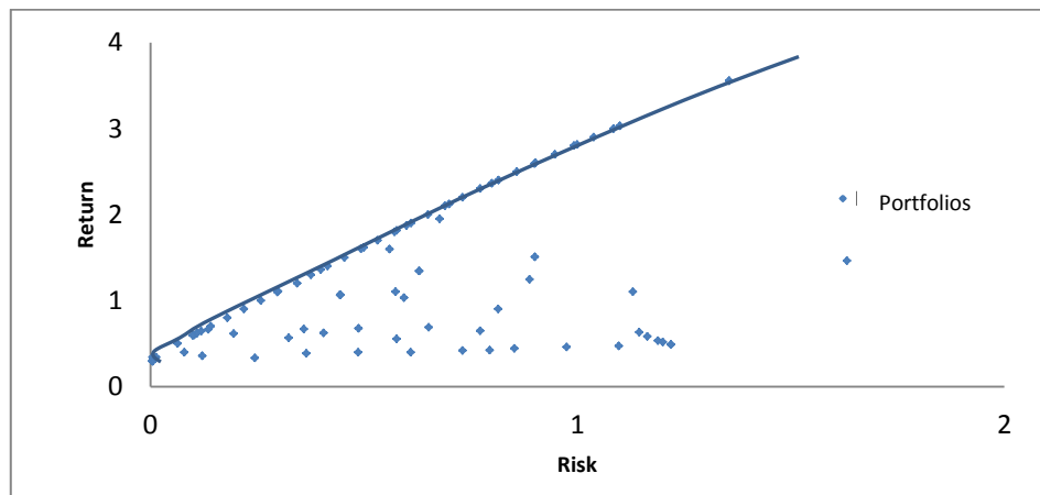
Figure 5. Efficient frontier 1
