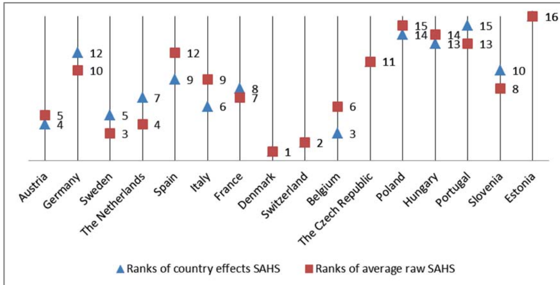
Figure 6: Ranks of country effects versus ranks of average country raw SAHSs
