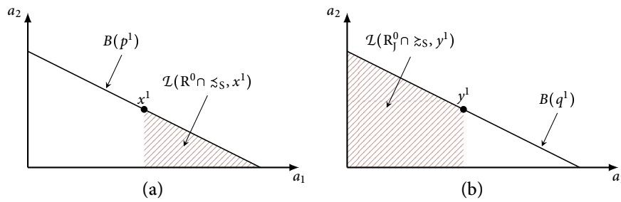
Figure 3: An illustration of \tilde{R}_J and \tilde{R} . In (a), we have x^1 R^0 a and x^1 z_S a for all a in the indicated region and thus x^1 \tilde{R}_J a . In (b), we have y^1 R_J^0 a and y^1 z_S a for all a in the indicated region and thus y^1 \tilde{R} a .
