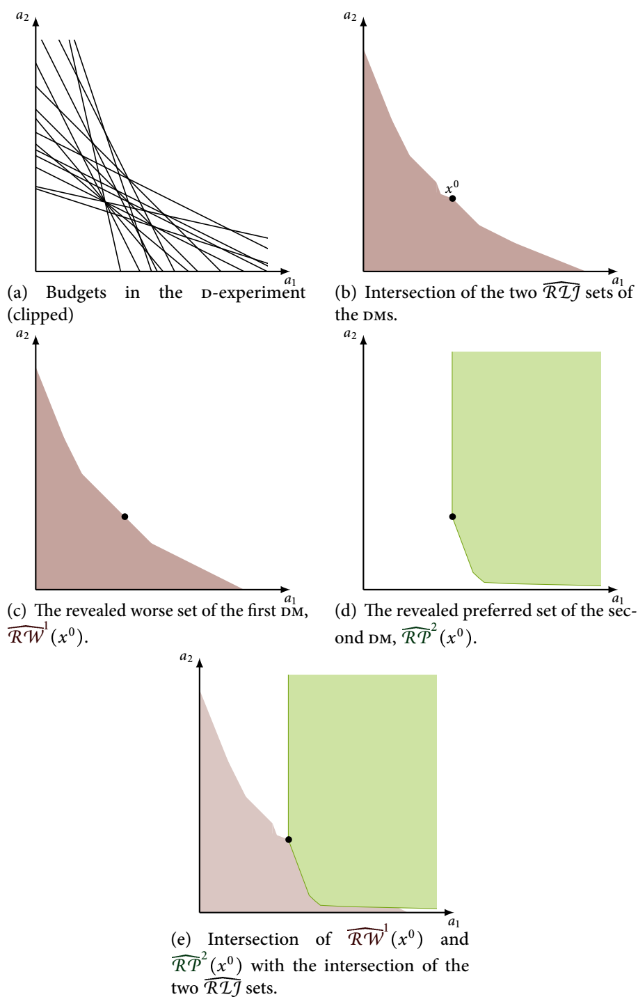
Figure 12: Sense of justice with revealed sets. Choices were generated on the budgets in (a) using two Cobb-Douglas utility functions with \alpha = 1\frac{1}{2}\% for DM^1 and \alpha = 1\frac{9}{10}\% for DM^2 . A similar set of budget was used for choices in a P- or v-experiment. Both DMS have the same symmetric Cobb-Douglas justice function. As the last figure clearly indicates, the first DM has a stronger revealed sense of justice than the second DM.
