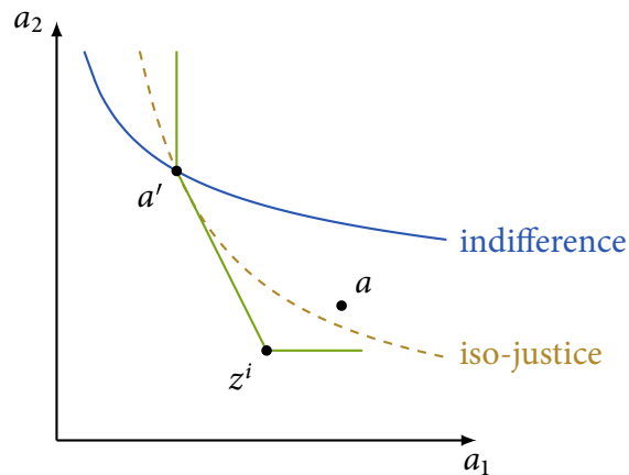
Figure 15: Illustrations for the proof of Theorem 2: If a \succ_S a' and u(a) \leq u(a') , then v(a) \leq v(a') is possible given AGGARP.
