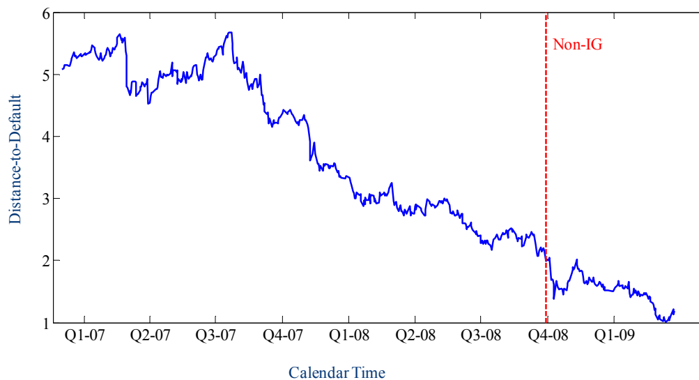
Figure 3: Development of the Distance-to-Default (DD) of Fiat Spa
