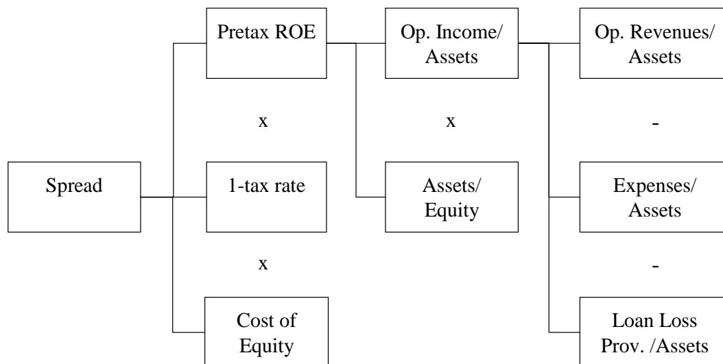
Figure 2: Spread Decomposition
