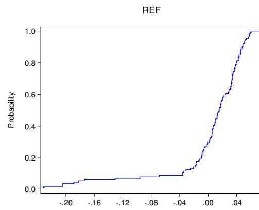
Figure 1: Empirical Cumulative Distribution Function \hat{F}(y_t)
