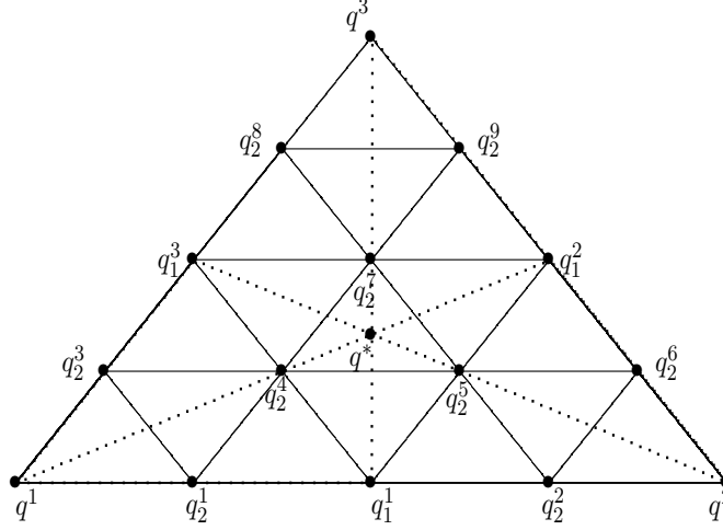
Figure 1: 1st and 2nd Simplicial partitions
