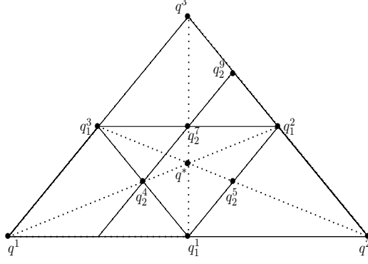
Figure 2: Step from 1st to 2nd Simplicial partition
