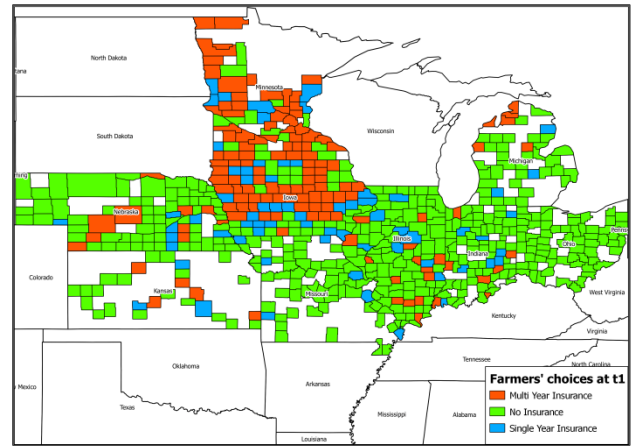
d: SY and MY distributions at t_1
