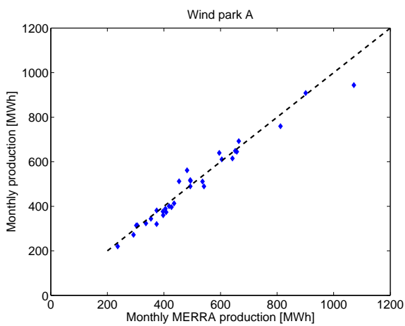
Figure 9: Monthly MERRA production vs. true monthly production
