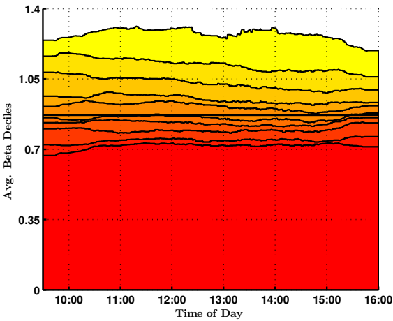
(a) Betas
