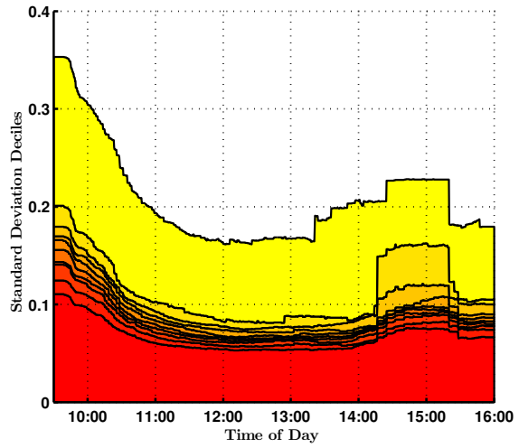
(b) Volatilities
