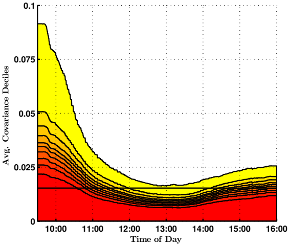
(a) Covariances
