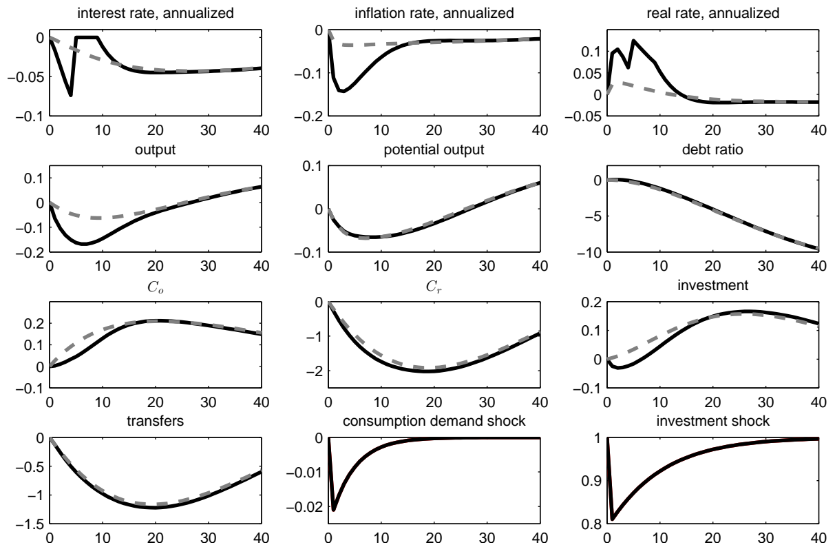
Figure 10: Transmission of consolidation via transfers at the ZLB. Notes: solid line : effect of consolidation at ZLB, dashed line : baseline.
