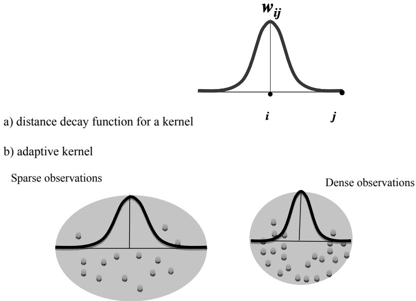
Figure 3.1: GWR spatial fixed and adaptive kernel
