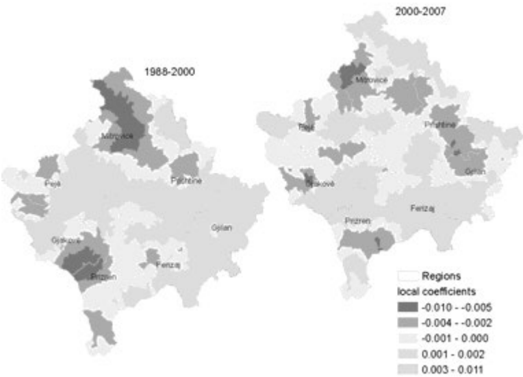
B) Distance to nearest highway
