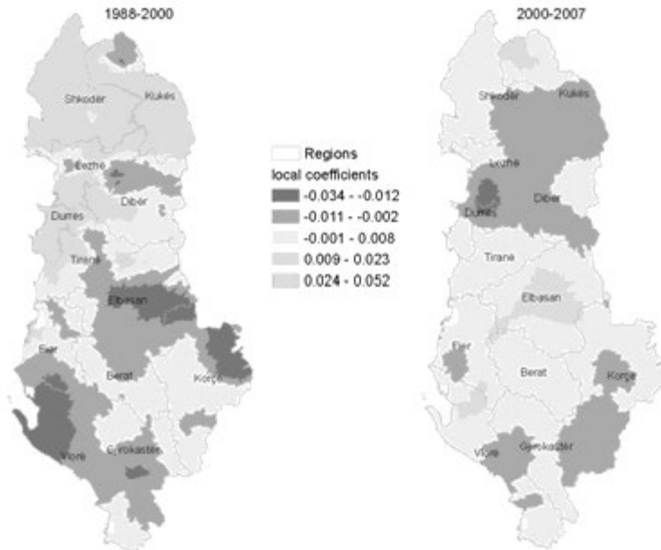
B) Distance to nearest major roads
