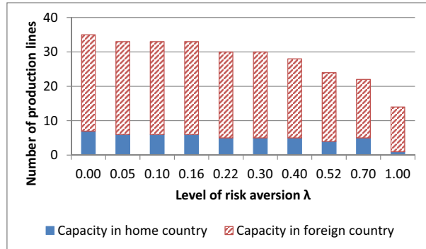
(b) ir_{C1} = 4\% , ir_{C2} = 7\% , with forwards and options
