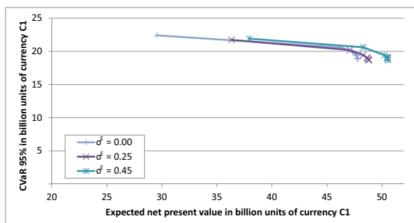
(e) No financial instruments, \alpha = 0.25
