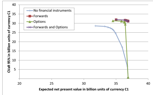
(b) \sigma^E = 0.45, \sigma^D = 0.05
