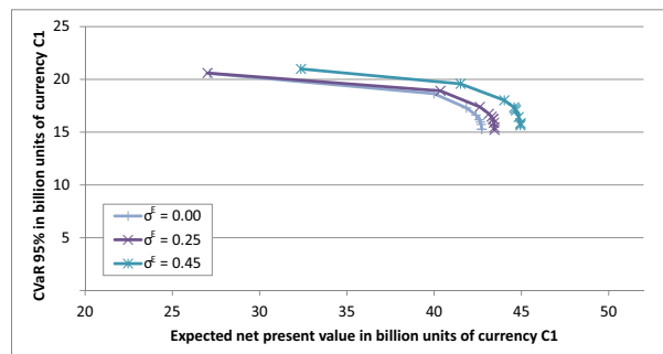
(d) With forwards and options, \alpha = 0.5
