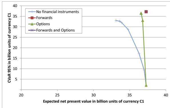
(a) \sigma^E = 0.45, \sigma^D = 0
