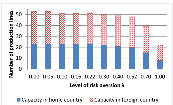
(h) With forwards and options, \sigma^E = 0.45 , \alpha = 0.25
